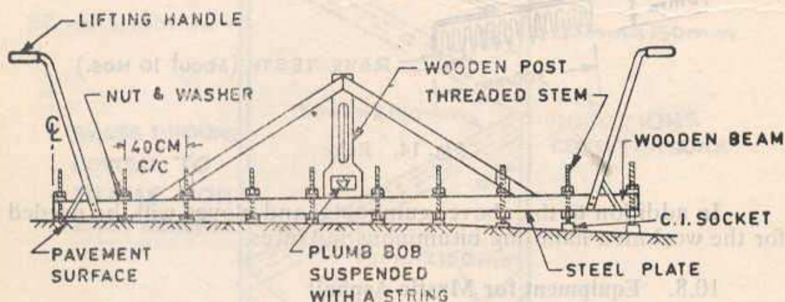
Fig. 15. One design of template with adjustable profile
