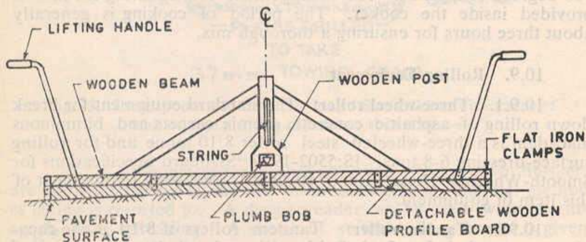
Fig. 16. Another design of template with adjustable profile
